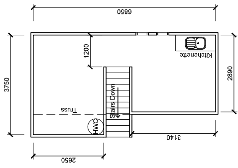
MEZZANINE FLOOR PLAN SCALE 1:100 - A3
